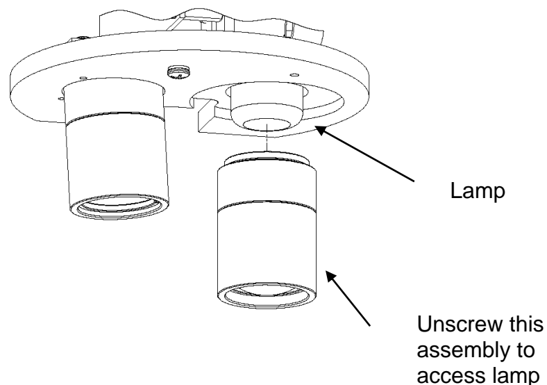
Figure 1 Flash Lamp
