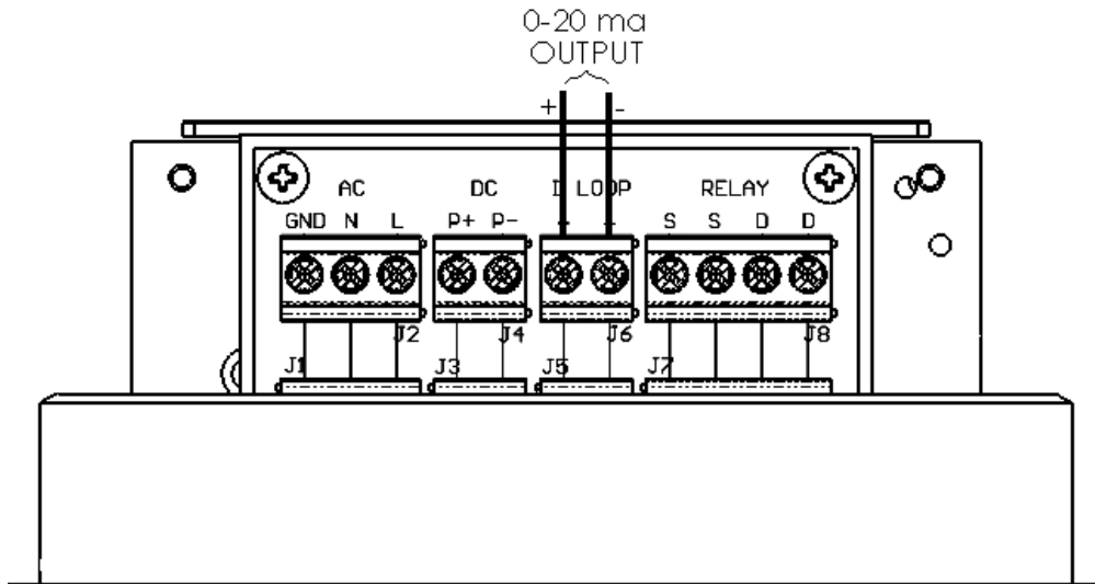
Figure 2.3-3 0-20ma Current Source Output Wiring
