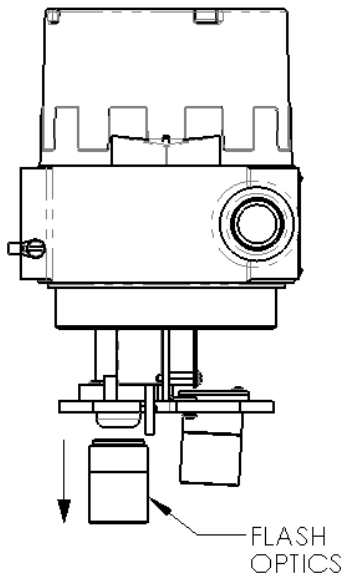
Figure 2 Flash Optics Replacement
