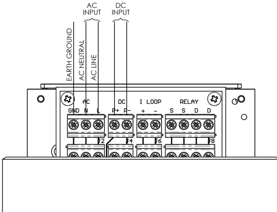
Figure 2.3-1 Power Wiring
