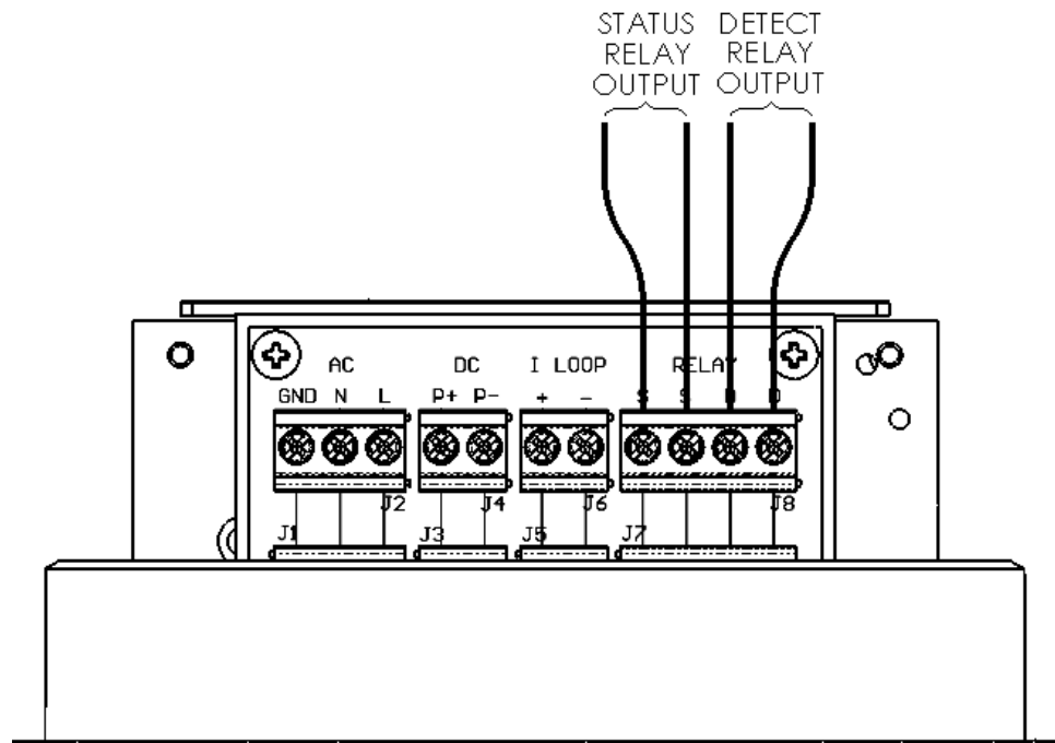
Figure 2.3-2 Relay Output wiring
